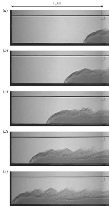
FIG. 2: Propagating dense current, with the total time taken for the front to propagate from frame (a) to frame (e) was 6.70s, where the distance between two consecutive frames was 0.20 m. With g' = 0.29 \text{ ms}^{-2} and H = 0.20 \text{ m} , these photos suggest that the front traveled at a constant speed of 0.5(g'H)^{1/2} .
