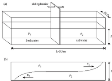
FIG. 1: (a) Laboratory apparatus used for experiments of lock-release gravity currents and (b) a simplified feature of a propagating gravity current in the channel.
